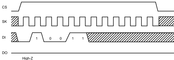
Fig.3 Write enable cycle timing
