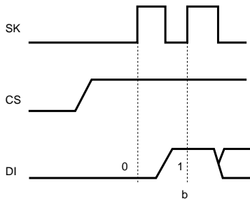
Fig.9 Timing during normal operation
