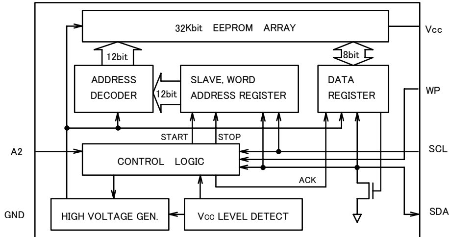
Figure 2. Block Diagram
