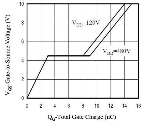
Figure8. Gate Charge
