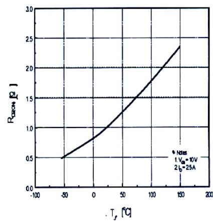
R_{DS(on)} - T_J
