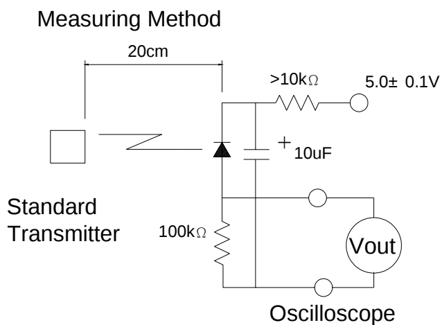
Fig.2 Measuring Method
