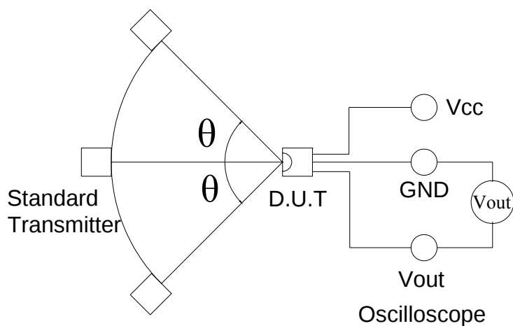
Fig.3 Measuring System
