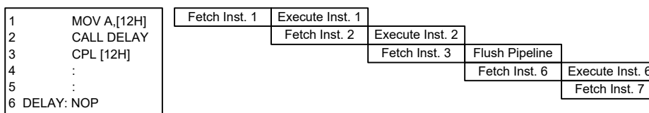
Instruction Fetching
