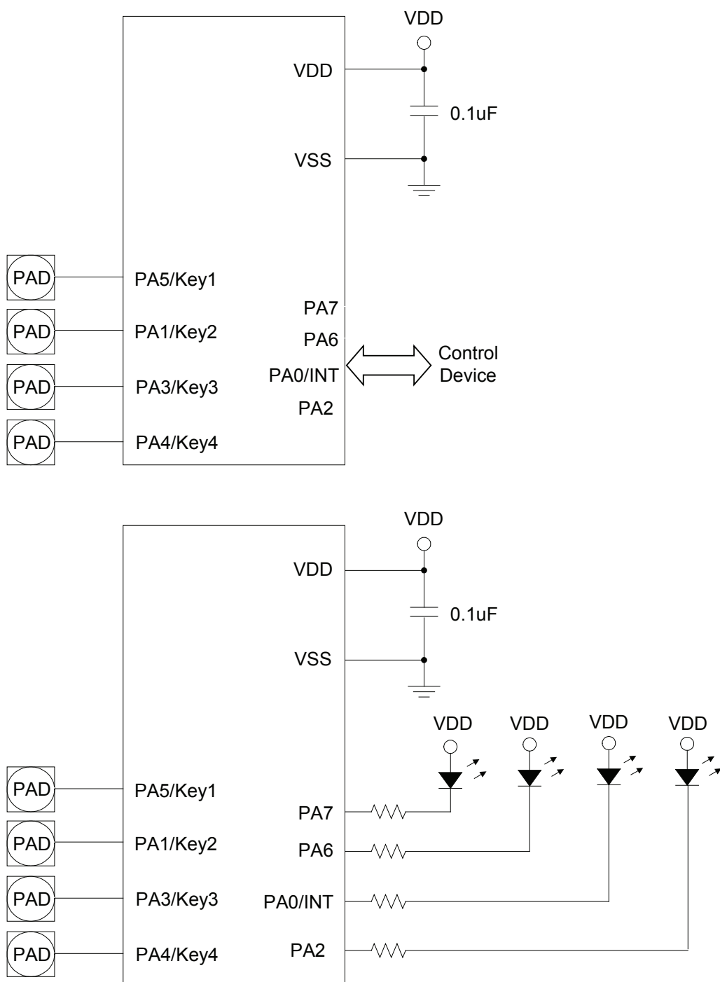
BS83A04A-3/BS83A04A-4
