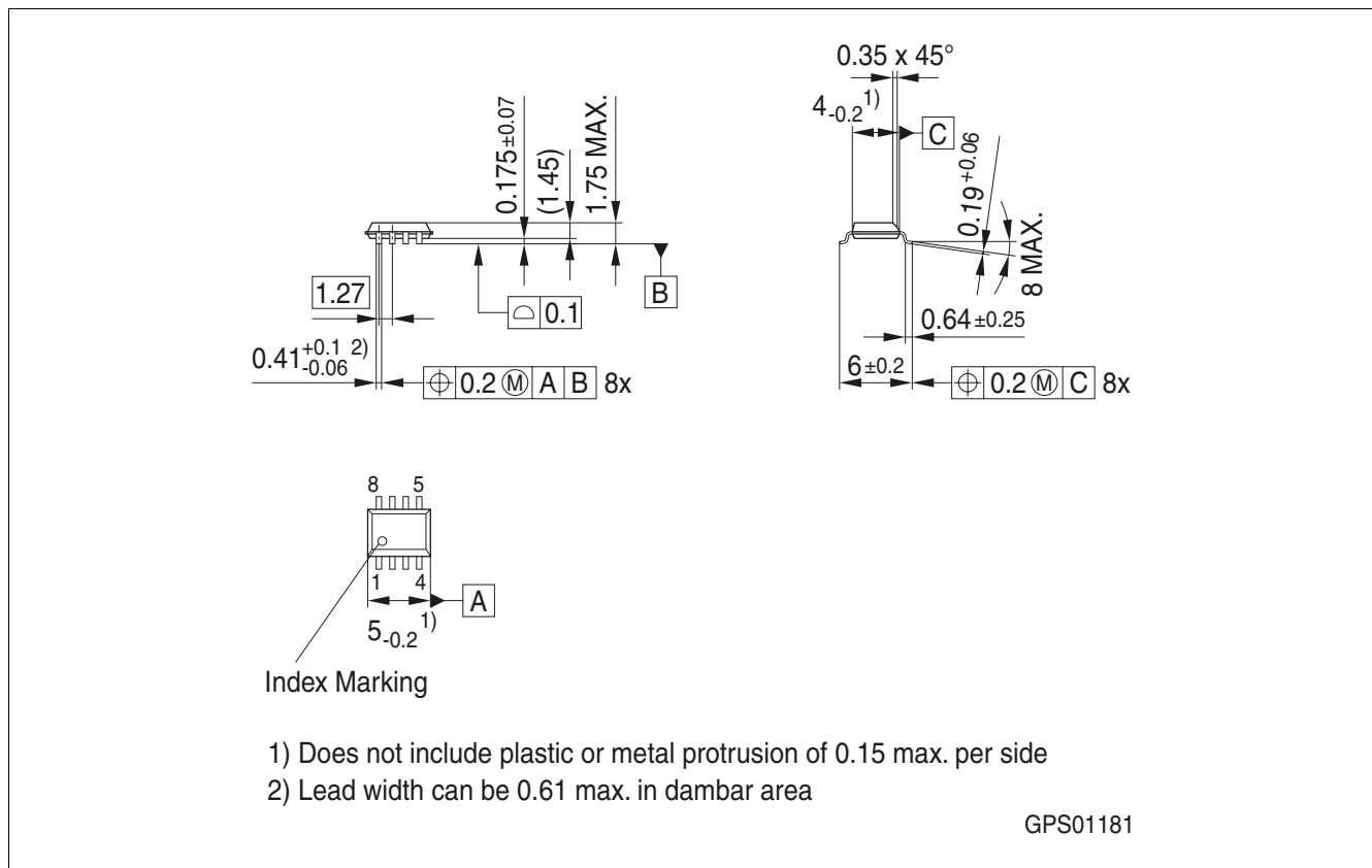
Figure 1 PG-DSO-8-25
