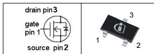
PG-SC-59
