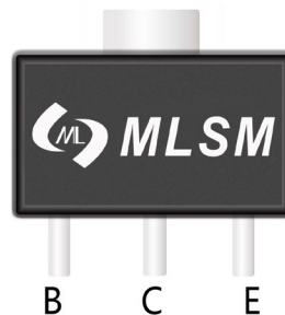
SOT-89-3L top view
