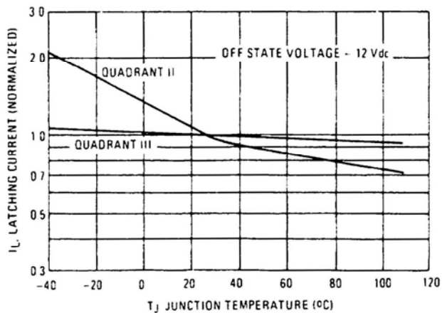
FIGURE 6 – TYPICAL LATCHING CURRENT
