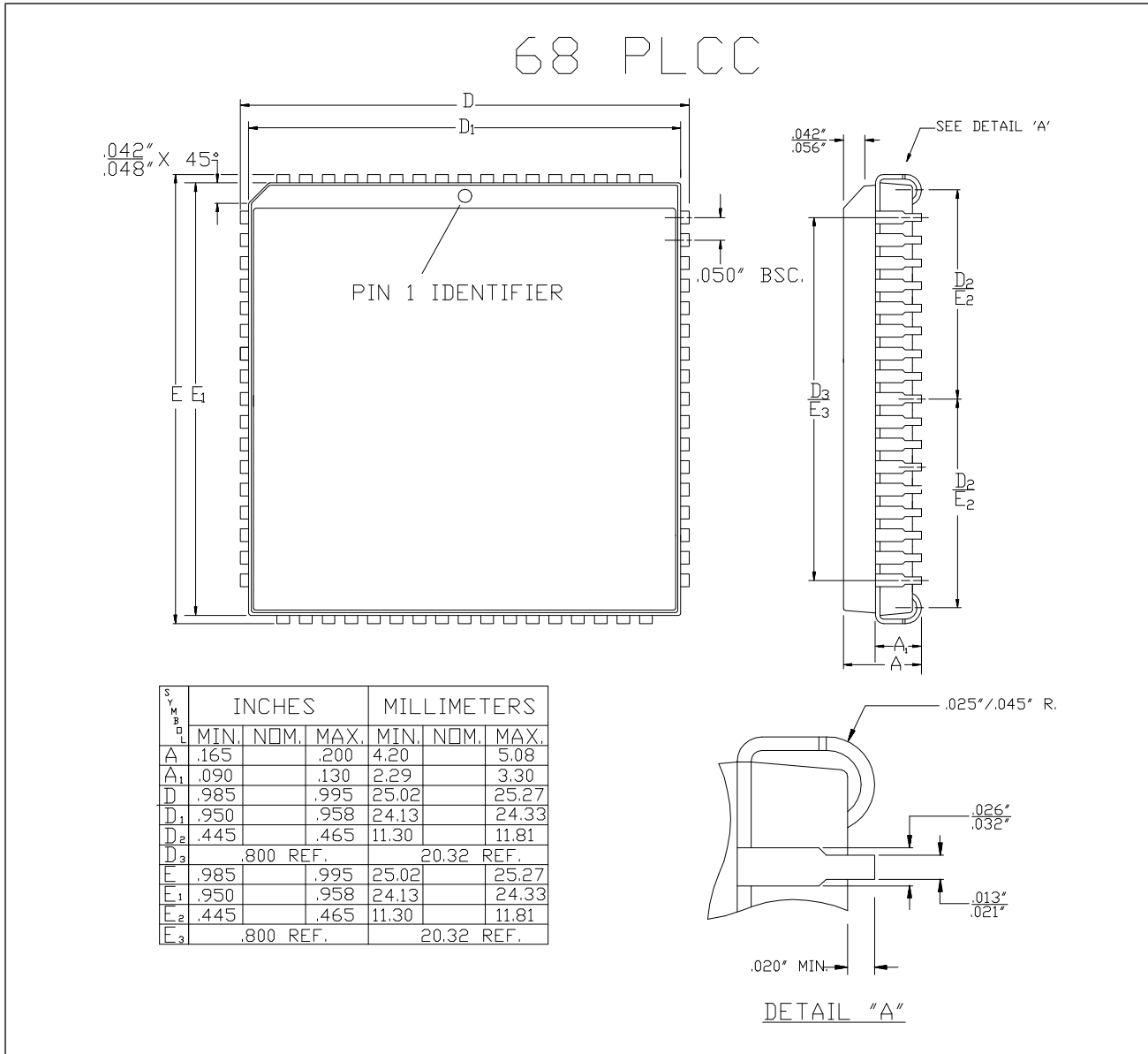
Figure 20. 68-Pin PLCC
