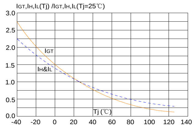
Fig.6: Relative variations of gate trigger current, holding current and latching current versus unjunction temperature
