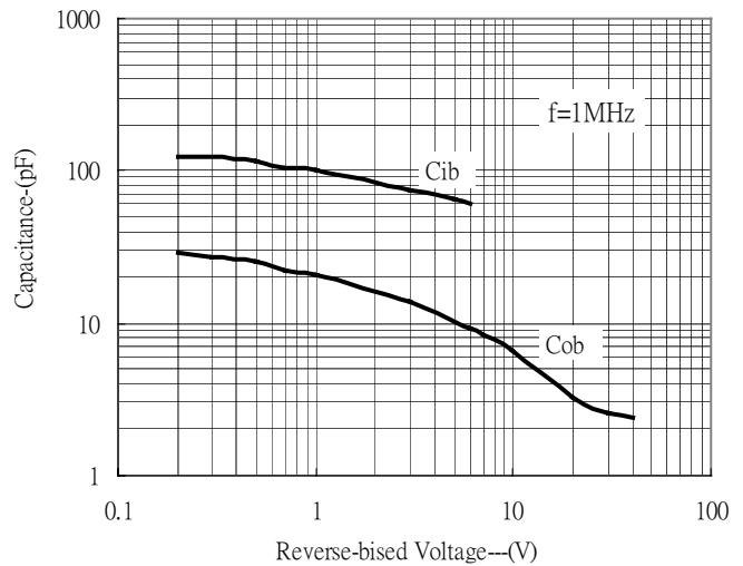
Capacitance Characteristics
