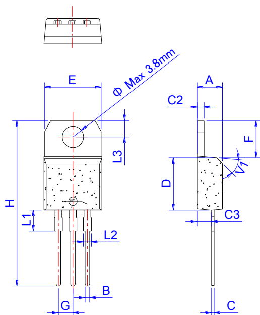
TO-220AB Non-Ins
