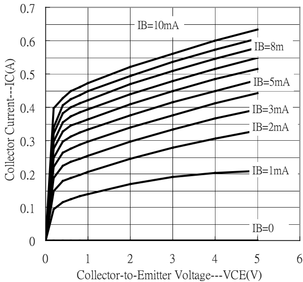
Output Characteristics
