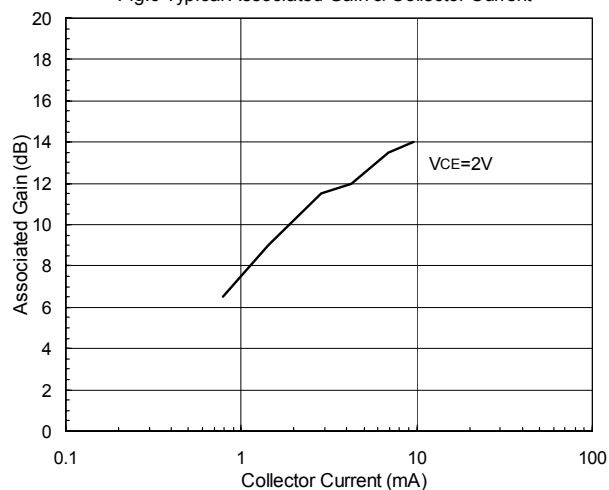
Fig.6 Typical Associated Gain & Collector Current
