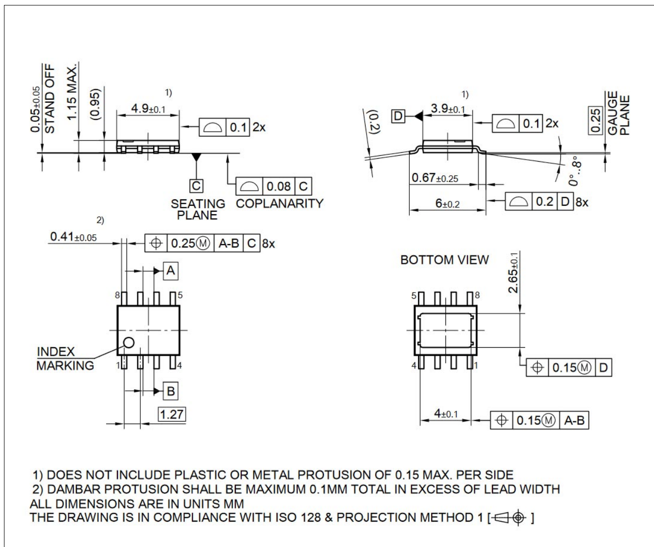
Figure 52 PG-TDSO-8-31 1)
