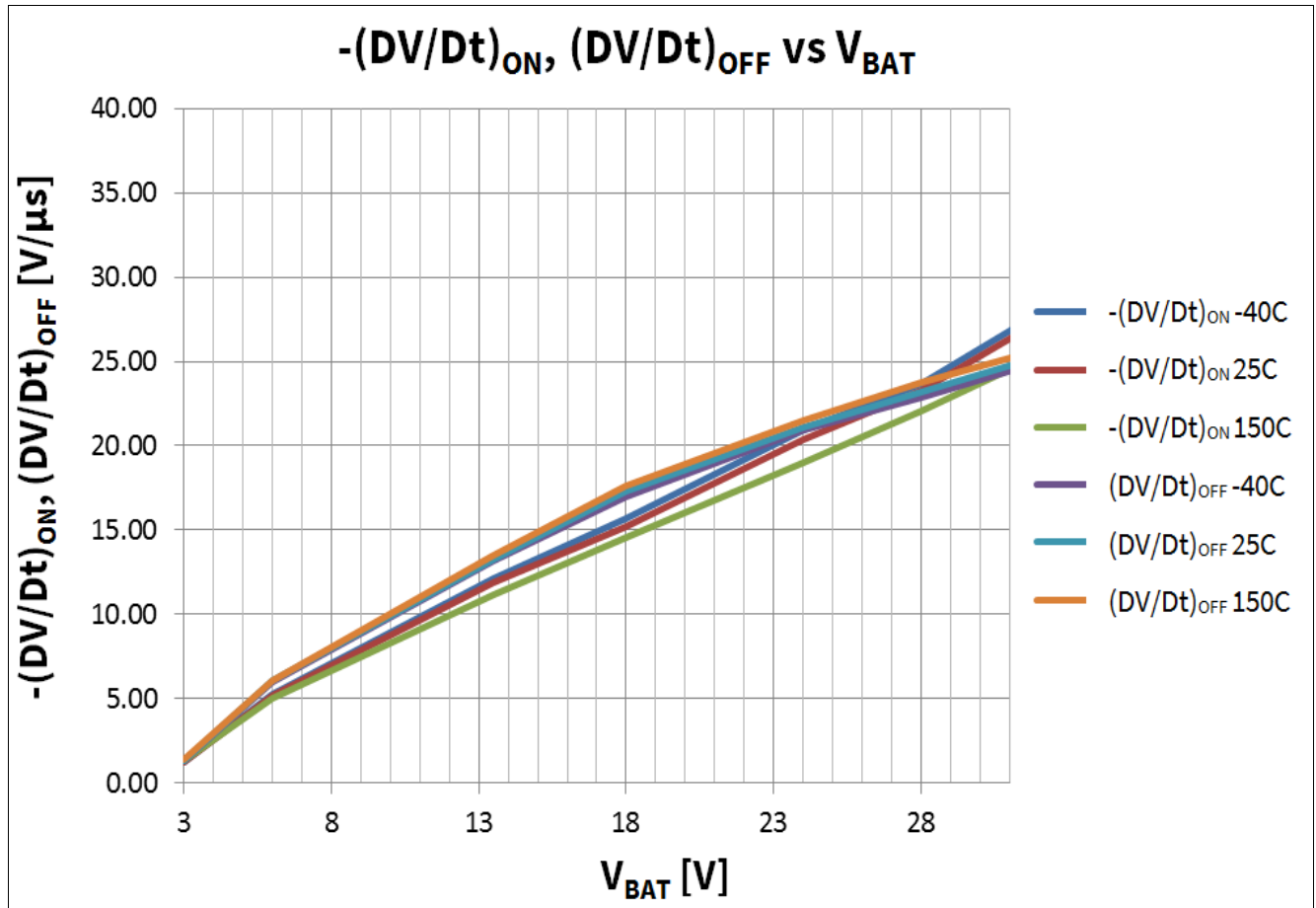
Figure 36 Slewrates -(DV/Dt)_{ON}, (DV/Dt)_{OFF} vs. V_{BAT} @ T_J = -40, 25, 150^\circ\text{C} ; R_L = 4.7\Omega ; R_{SRP} = 5.8\text{k}\Omega ; V_{IN} = V_{DD} = V_{ENABLE} = 5\text{V} ; V_{BAT} = 3..31\text{V}
