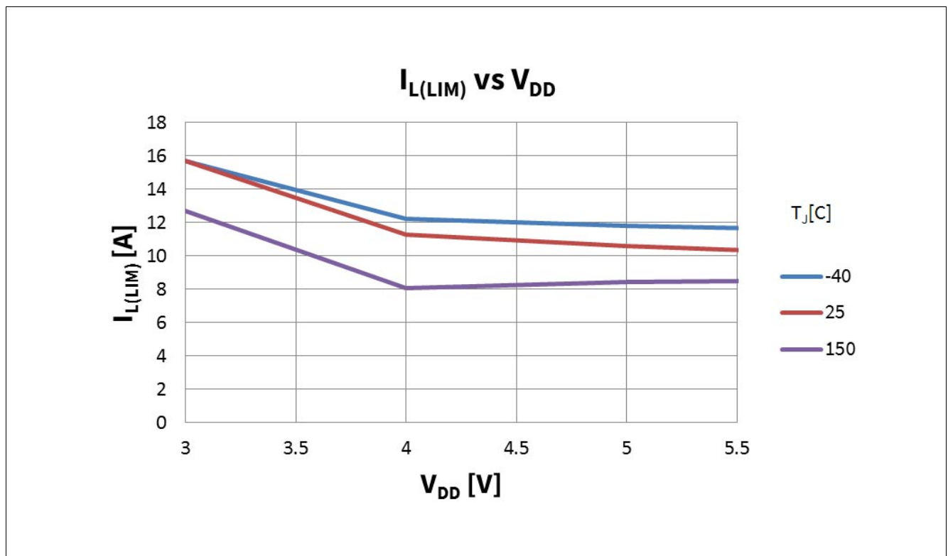
Figure 42 I_{L(LIM)} vs. V_{DD} = 3\text{V}...5.5\text{V} @ T_J = -40, 25, 150^\circ\text{C} ; V_{ENABLE} = V_{IN} = 5\text{V} ; V_{BAT} = 13.5\text{V}
