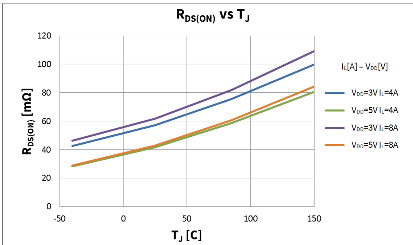
Figure 26 R_{DS(ON)} vs. T_J @ V_{DD}=3\text{V}, 5\text{V} ; V_{IN} = V_{ENABLE} = 5\text{V} ; T_J = -40, 25, 85, 150^\circ\text{C}
