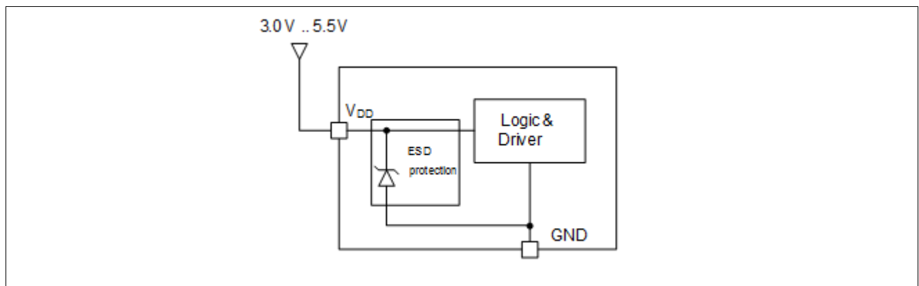
Figure 21 Supply Circuit
