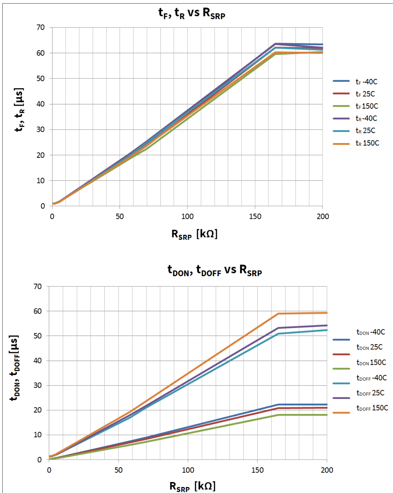
Figure 32 t_F, t_R, t_{DON}, t_{DOFF} vs. R_{SRP} ; V_{IN} = V_{ENABLE} = V_{DD} = 5V ; V_{BAT} = 13.5V ; R_L = 4.7\Omega ; T_J = -40, 25, 150^\circ C
