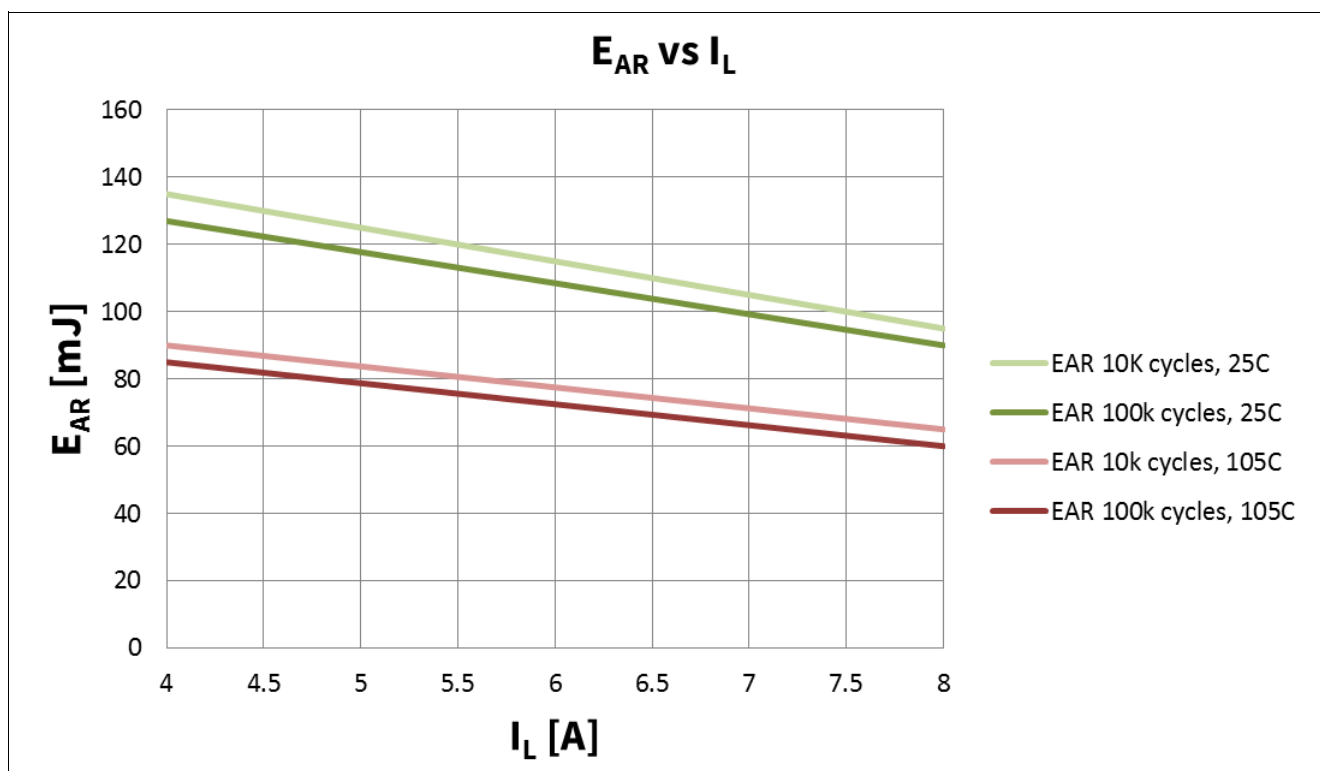
Figure 30 E_{AR\_10k, \_100k} vs. I_L @ T_{J(0)}=25^\circ\text{C}, 105^\circ\text{C}, V_{BAT} = 13.5\text{V}; V_{IN} = V_{ENABLE} = V_{DD} = 5\text{V}; I_L = I_{L(NOM)}/4, I_{L(NOM)}/2, I_{L(NOM)}, 2 \cdot I_{L(NOM)}
