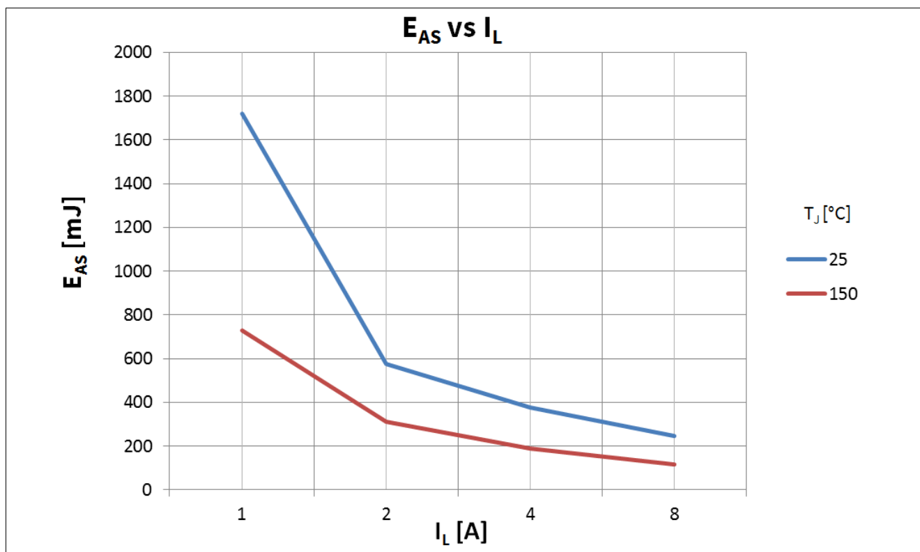
Figure 29 E_{AS} vs. I_L @ T_{J(0)}=25^\circ\text{C}, 150^\circ\text{C}, V_{BAT}=13.5\text{V}; V_{IN} = V_{ENABLE} = V_{DD} = \text{open}; I_L = I_{L(NOM)}/4, I_{L(NOM)}/2, I_{L(NOM)}, 2 \cdot I_{L(NOM)}
