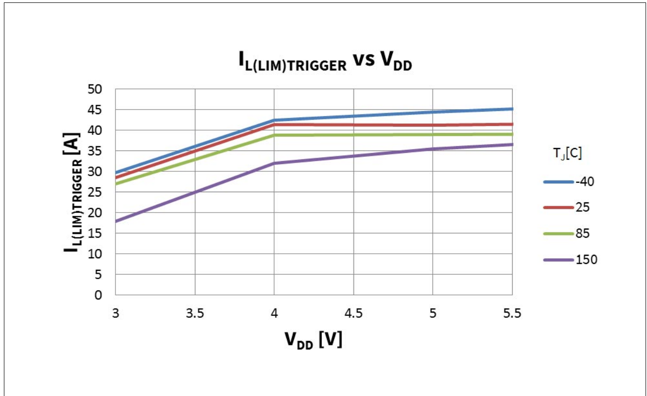
Figure 41 I_{L(LIM)TRIGGER} peak vs. V_{DD}=3...5.5\text{V} @ T_J = -40, 25, 85, 150^\circ\text{C} ; V_{IN} = \text{PWM } 5\text{V} in SOA; V_{ENABLE} = 5\text{V} ; V_{BAT} = 13.5\text{V} ; R_L = 4.7\Omega
