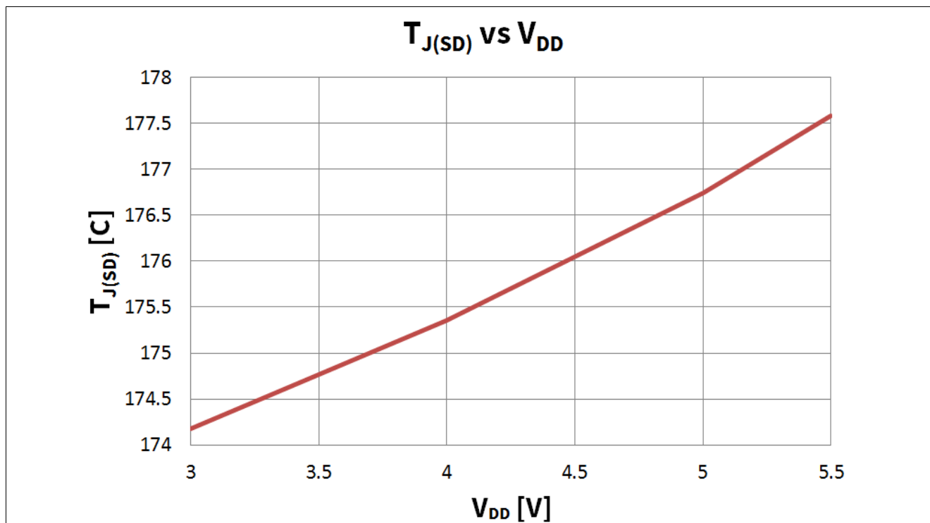
Figure 39 T_{J(SD)} vs. V_{DD} ; V_{IN}=V_{ENABLE}=5V ; V_{DD}=3V...5.5V ; I_L=10mA
