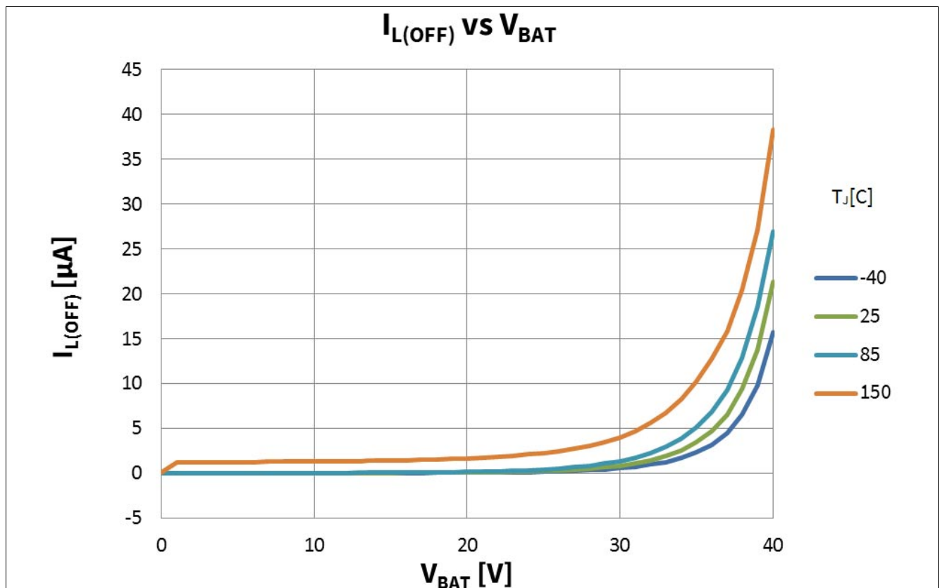
Figure 28 I_{L(off)} vs. V_{BAT}=0..40V @ T_J=-40, 25, 85, 150^{\circ}C ; V_{IN}=0V ; V_{ENABLE}=V_{DD}=5V
