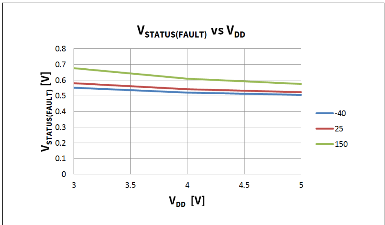
Figure 44 V_{\text{STATUS}} in fault mode vs. V_{\text{DD}} = 3\text{V} \dots 5\text{V} @ T_{\text{J}} = -40, 25, 150^\circ\text{C} ; V_{\text{IN}} = V_{\text{ENABLE}} = 5\text{V} ; V_{\text{BAT}} = 13.5\text{V} ;
