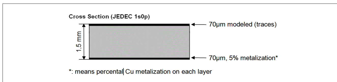
Figure 5 1s0p PCB Cross Section
