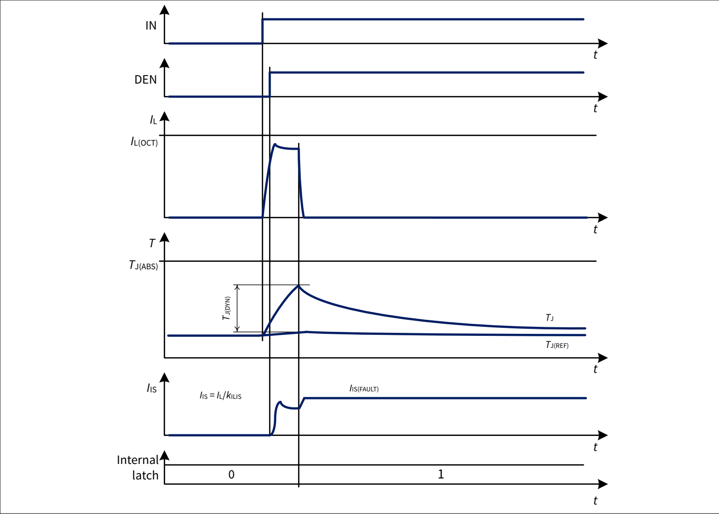
Figure 26 Overtemperature protection (dynamic)
