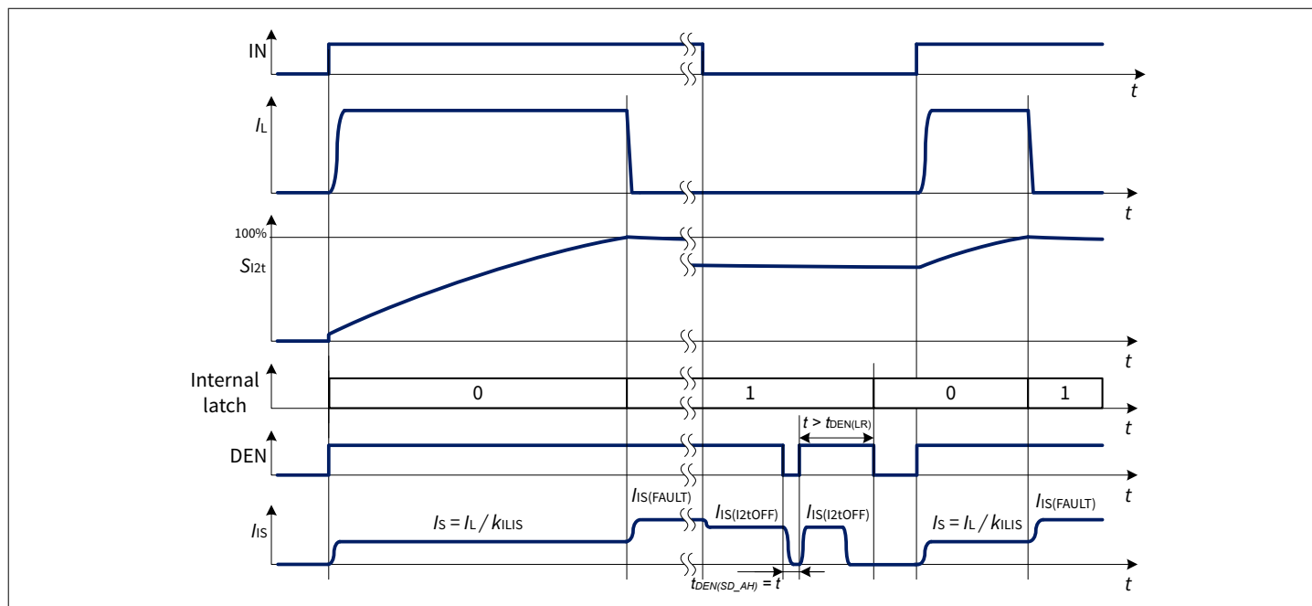
Figure 39 Intelligent latch timing diagram for DEN reset in case of triggered I2t protection
