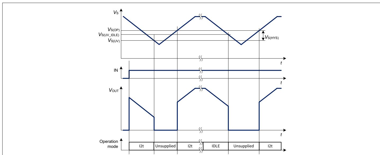
Figure 17 V_S undervoltage behavior
