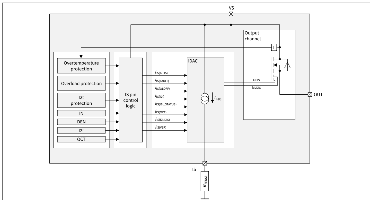
Figure 41 Diagnosis block diagram
