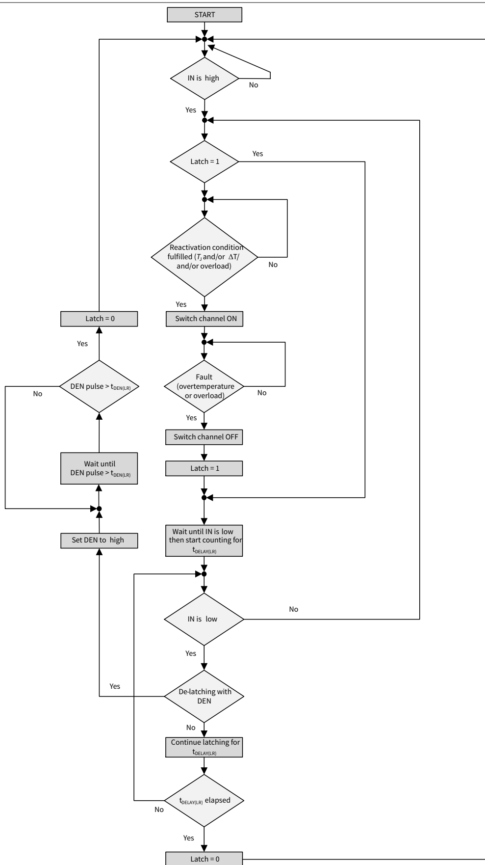
Figure 33 Intelligent latch flowchart in case of triggered device protection
