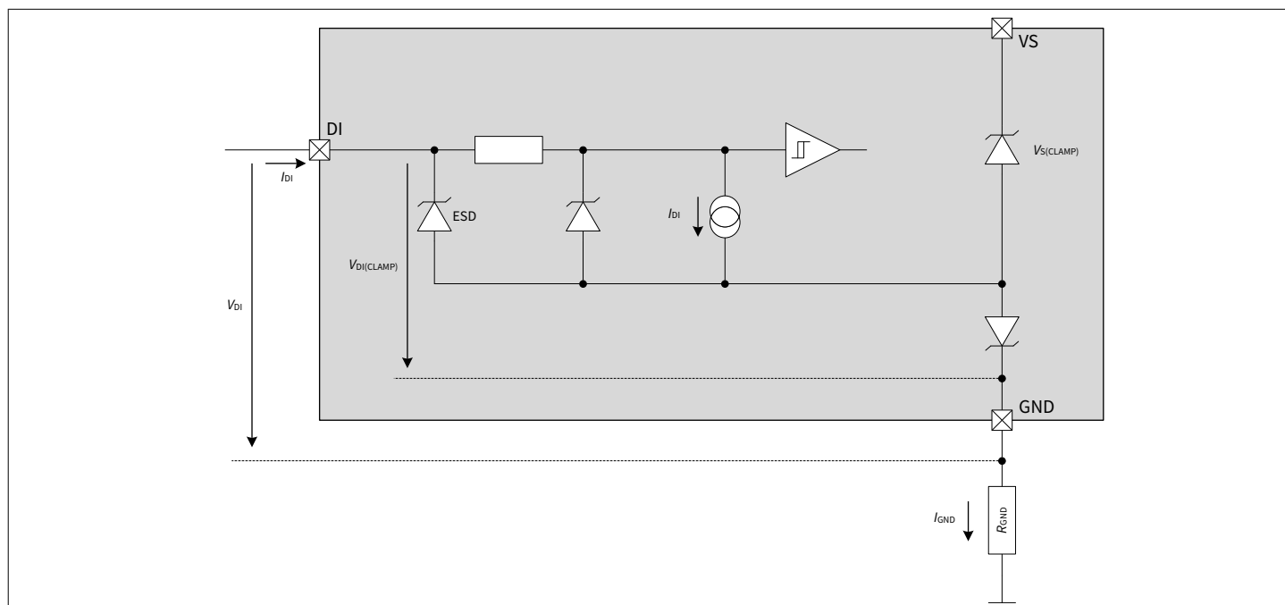
Figure 11 Input circuitry
