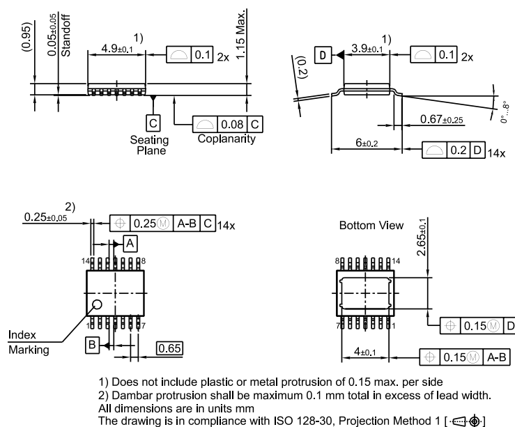
Figure 38 PG-TSDSO-14 dual small outline package dimensions
