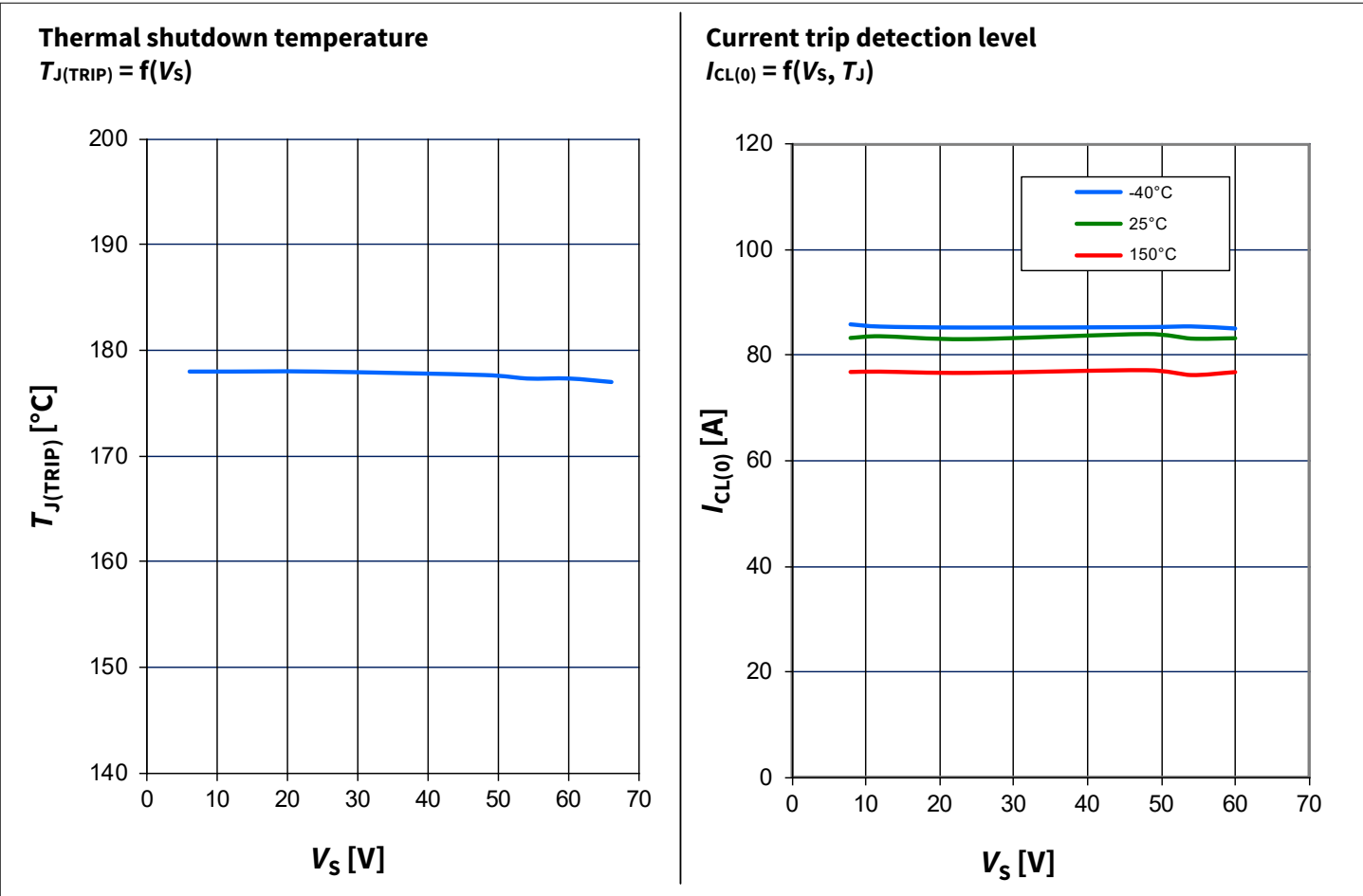
Figure 29 Typical performance characteristics (continued)
