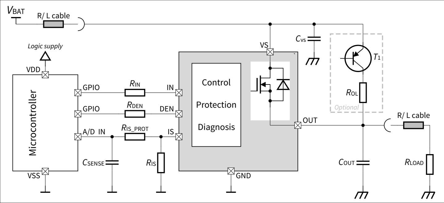
Application diagram
