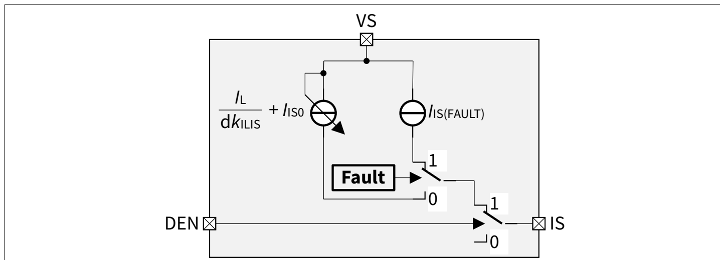
Figure 18 Diagnosis block diagram
