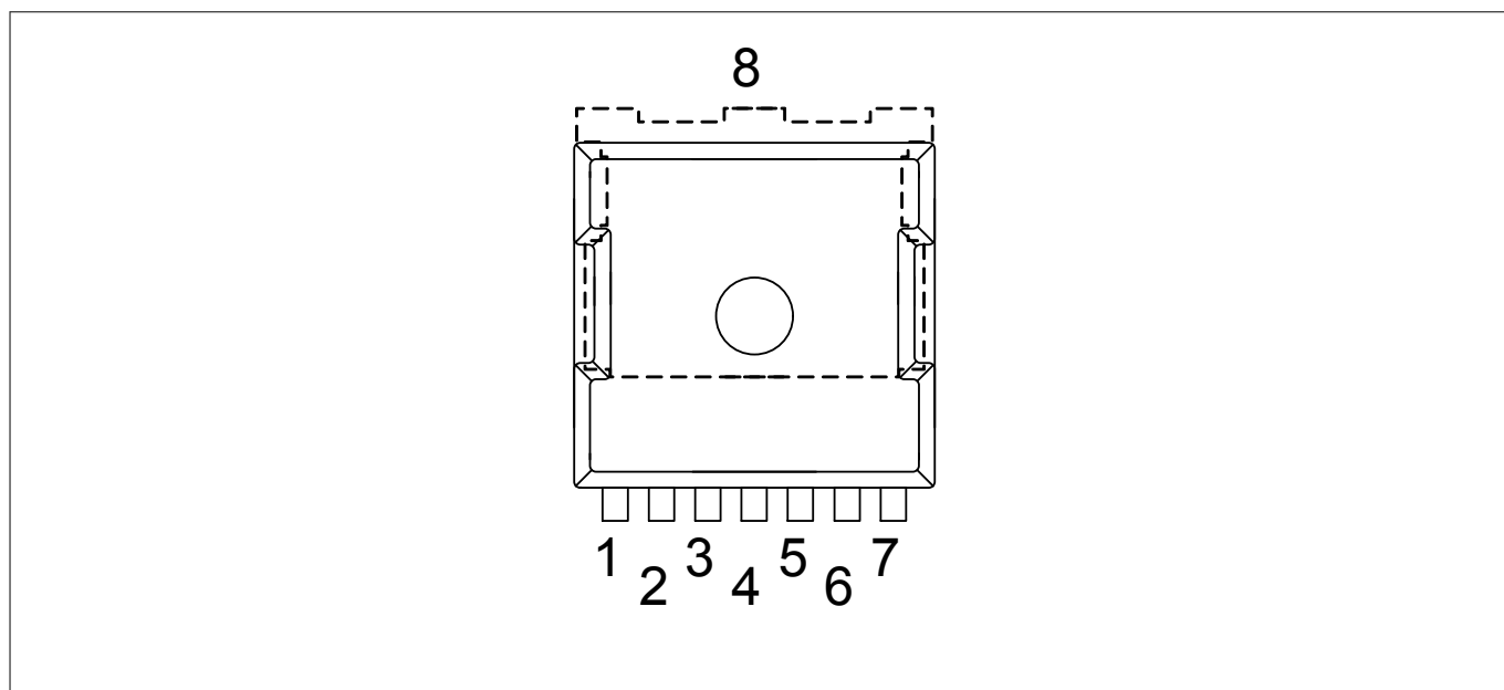
Figure 4 Pin assignment BTN9970LV (top view)
