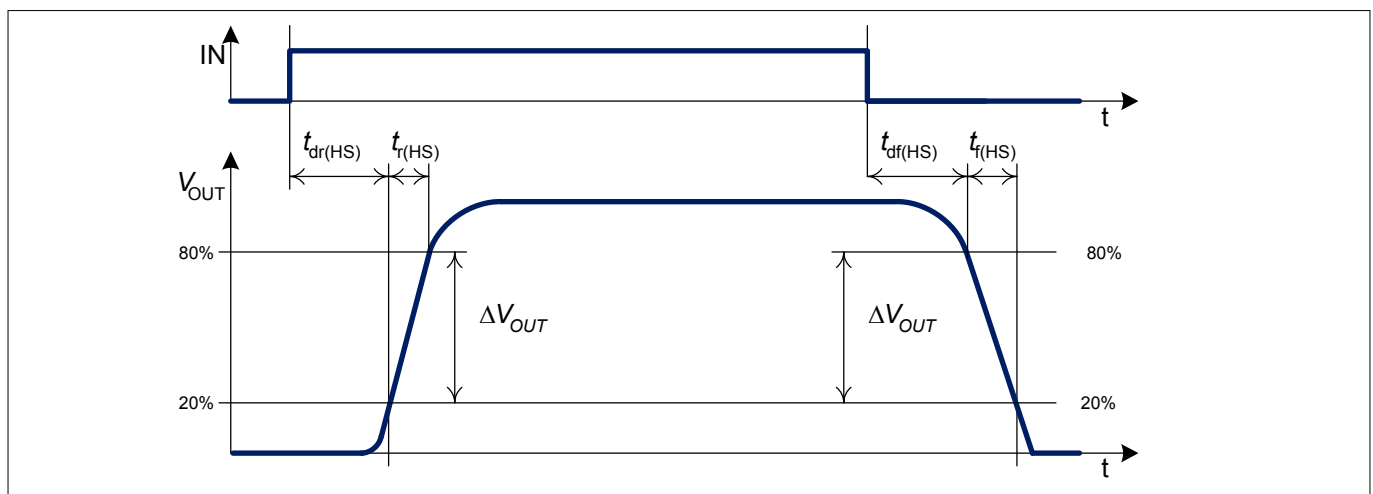
Figure 8 Definition of switching times high-side ( R_{\text{load}} to GND)
