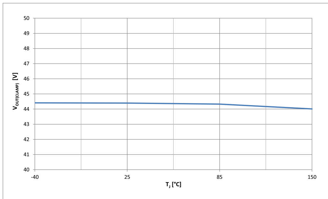
Figure 37 Typical V_{OUT(CLAMP)} vs. T_J @ I_L = 6 mA
