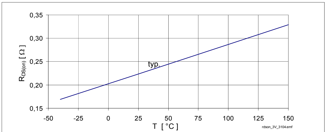
Figure 10 Typical On-State Resistance, R_{DS(on)} = f(T_J) , V_{IN} = 3V
