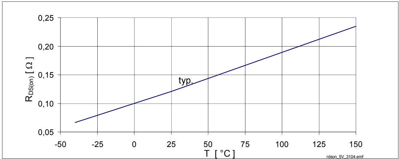
Figure 9 Typical On-State Resistance, R_{DS(on)} = f(T_J) , V_{IN} = 5V
