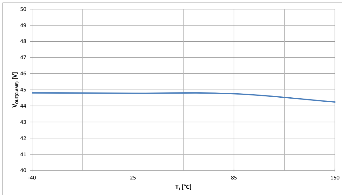
Figure 37 Typical V_{OUT(CLAMP)} vs. T_J @ I_L = 4 mA
