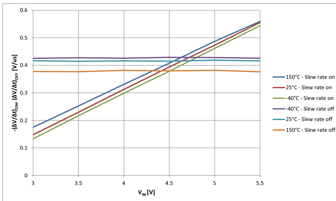
Figure 27 Typical -(\Delta V/\Delta t)_{ON} , (\Delta V/\Delta t)_{OFF} vs. V_{IN} @ T_J = -40 \dots 150^\circ\text{C}
