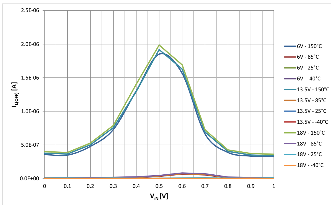
Figure 21 Typical I_{L(OFF)} vs. V_{IN} @ T_J = -40 \dots 150^\circ\text{C} , V_{BAT} = 6 \dots 18 \text{ V}
