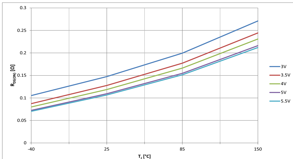
Figure 18 Typical R_{DS(ON)} vs. T_J @ V_{IN} = 3 \dots 5.5 \text{ V} , I_L = I_{L(NOM)}
