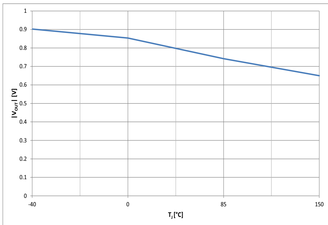
Figure 19 Typical Reverse Diode |V_{OUT}| vs. T_J @ I_L = I_{L(NOM)}
