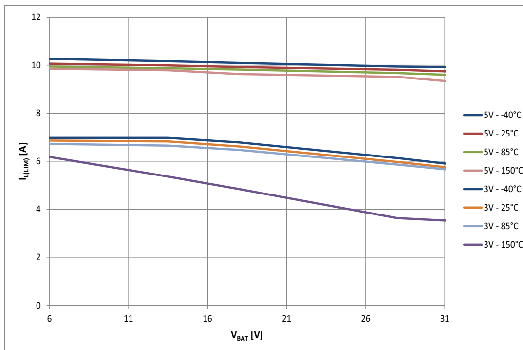
Figure 38 Typical I_{L(LIM)} vs. V_{BAT} @ T_J = -40 \dots 150^\circ\text{C} , V_{IN} = 3 V and 5 V
