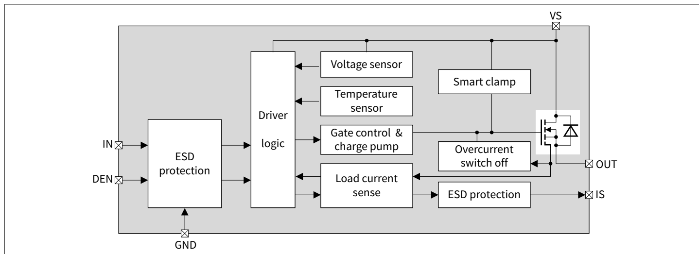
Figure 2 Block diagram
