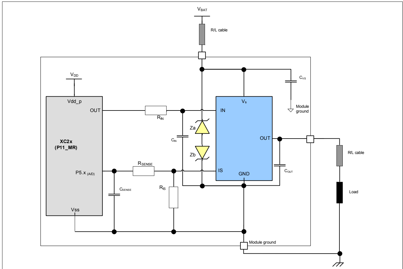
Figure 51 Application Diagram with BTS50015-1TAC
