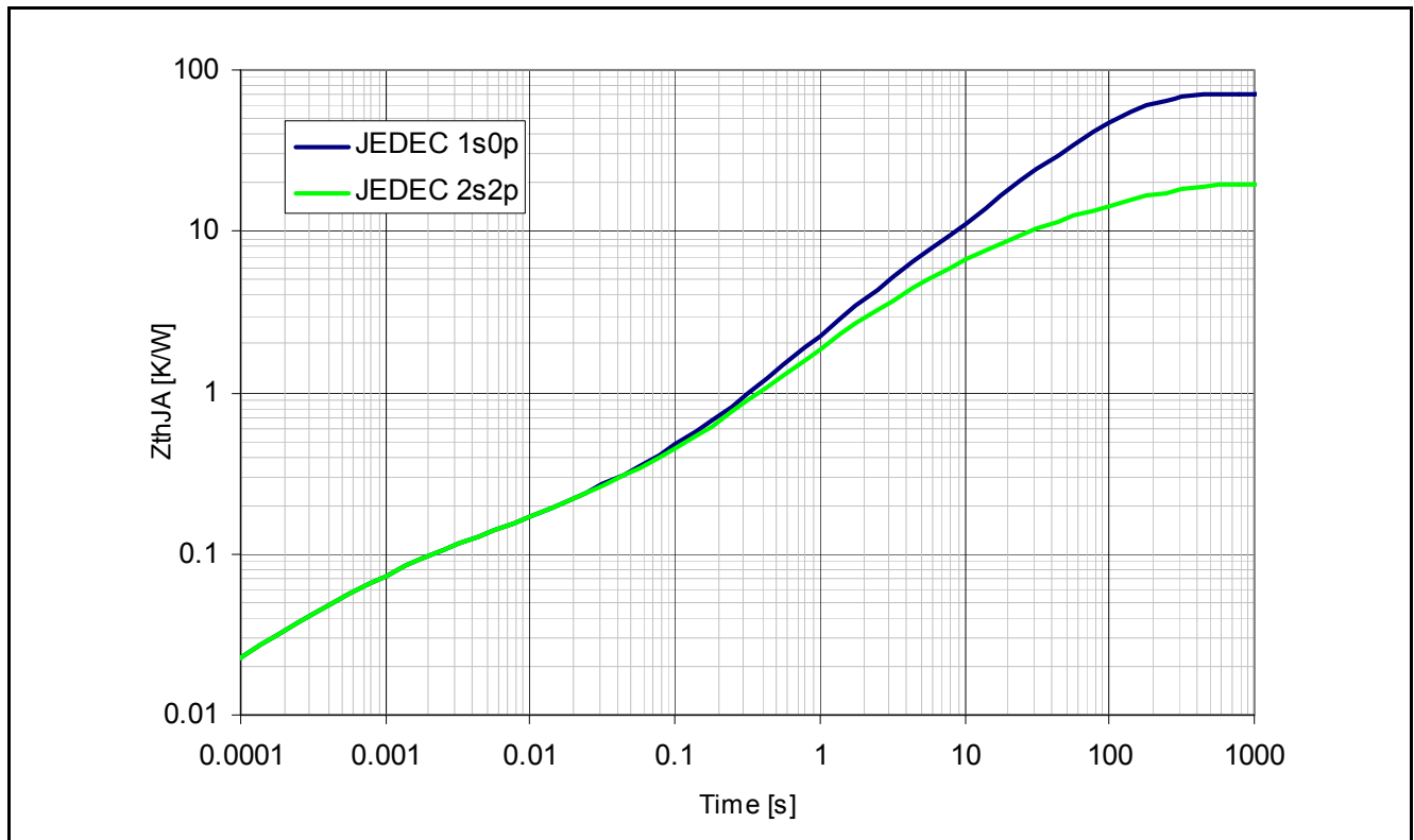
Figure 7 Typical Transient Thermal Impedance Z_{th(JA)} =f(time) for Different PCB Conditions
