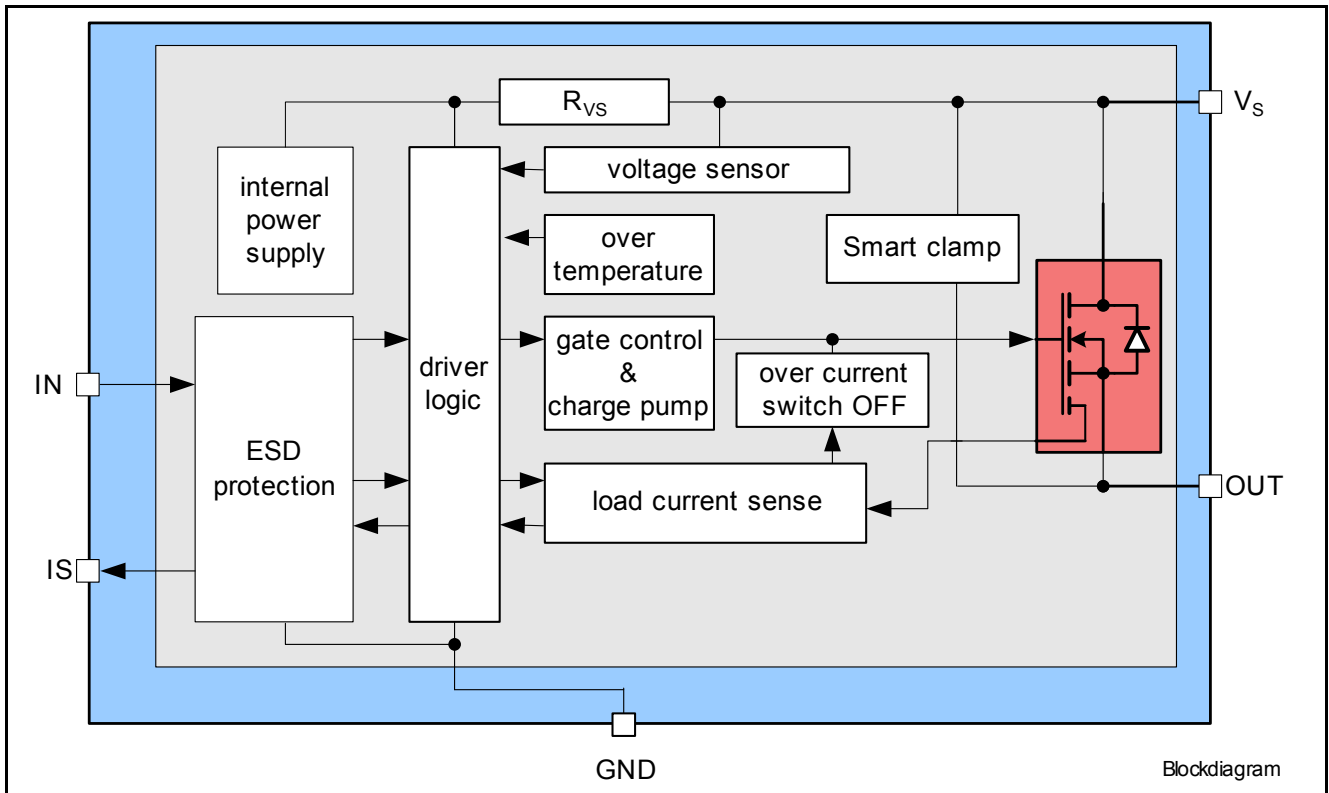
Figure 1 Block Diagram for the BTS50015-1TAC
