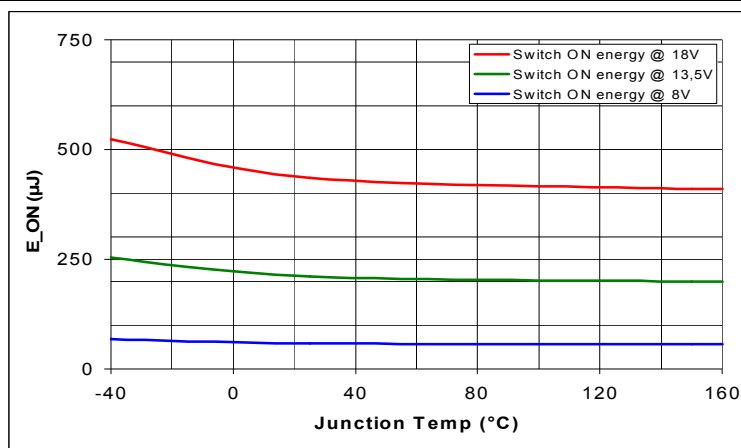
Figure 41 Switch ON Energy E_{ON} = f(T_J; V_S) , R_L = 12 \Omega
