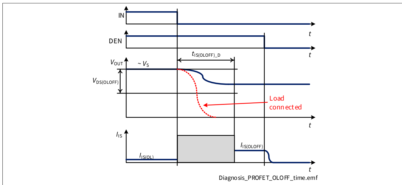
Figure 37 Open Load in OFF Timings - load disconnected
