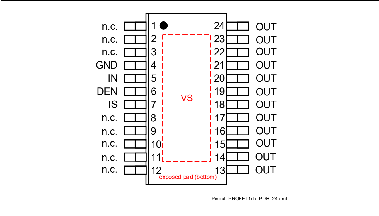
Figure 4 Pin Configuration
