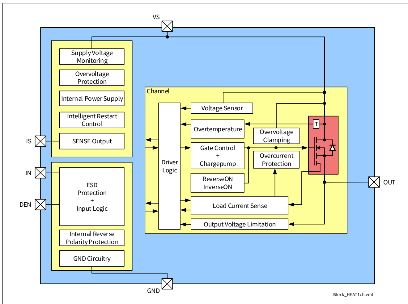
Figure 2 Block Diagram of BTS70015-1ESP
