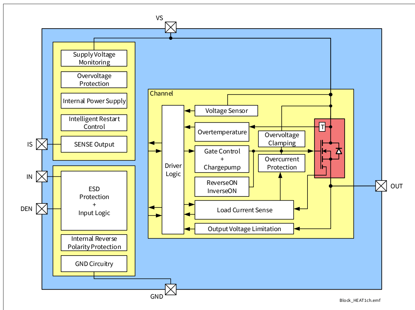
Figure 2 Block Diagram of BTS7002-1EPP
