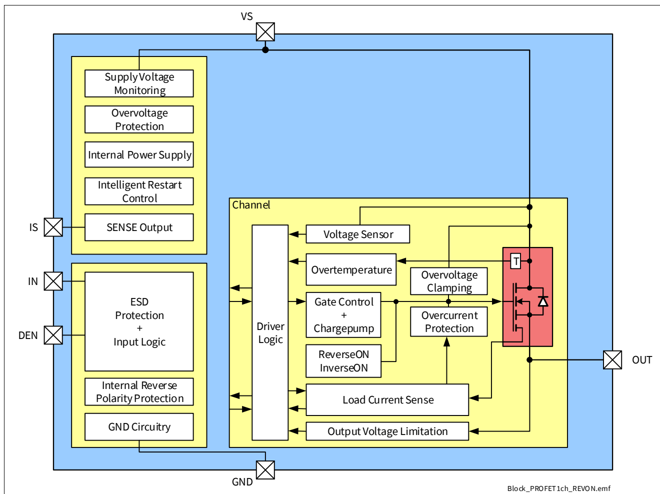
Figure 2 Block Diagram of BTS7010-1EPA
