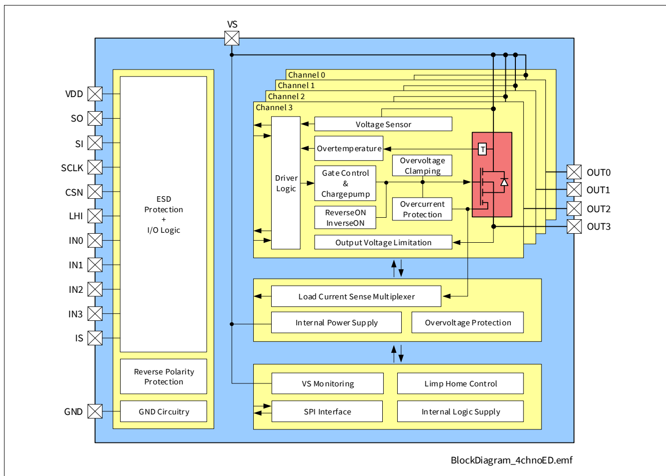
Figure 2 Block Diagram of BTS71220-4ESP
