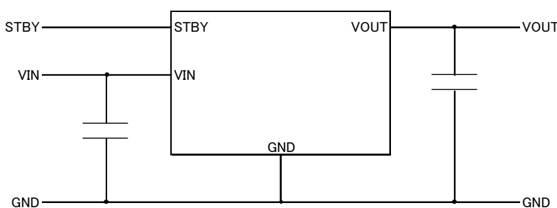
Fig.1 Application Circuit
