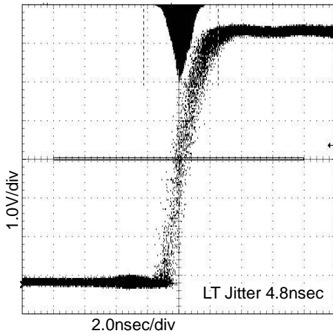
Figure 19 24.6MHz LT Jitter (V DD =3.3V, at C L =15pF)
