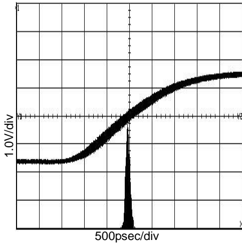
Figure 17. 27MHz Period-Jitter (V DD =3.3V, at C L =15pF)
