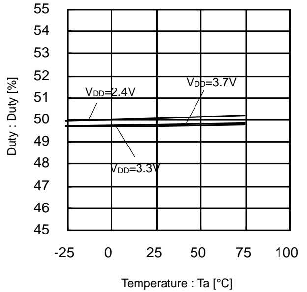
Figure 30. Duty vs Temperature (24.6MHz)
