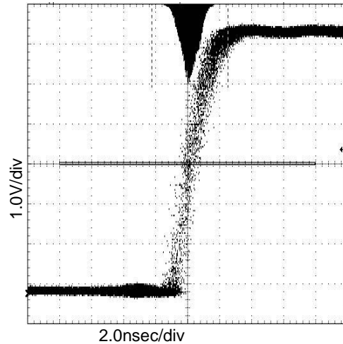
Figure 20. 22.6MHz LT Jitter (V DD =3.3V, at C L =15pF)
