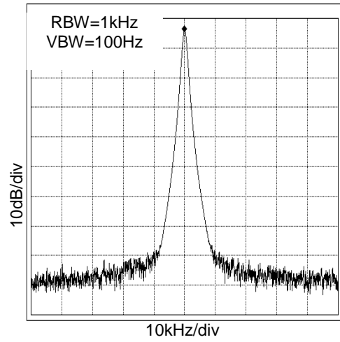
Figure 18. 27MHz Spectrum (V DD =3.3V, at C L =15pF)
