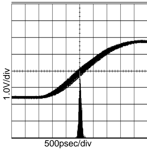
Figure 20. 27MHz Period-Jitter V_{DD}=3.3V , at C_L=15pF
