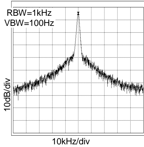
Figure 18. 18.4MHz Spectrum V_{DD}=3.3V , at C_L=15pF
