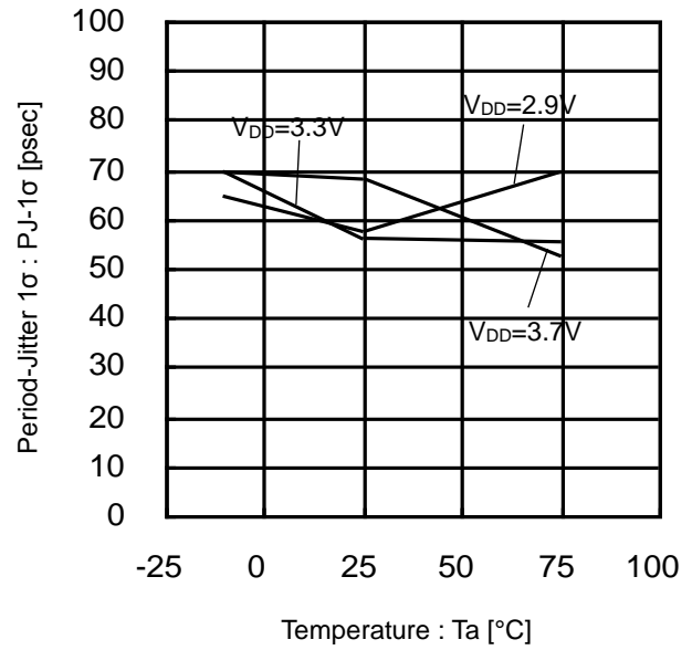
Figure 25. Period-Jitter 1σ vs Temperature (33.9MHz)
