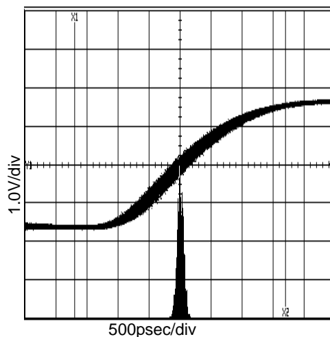
Figure 14. 22.6MHz Period-Jitter V_{DD}=3.3V , at C_L=15pF
