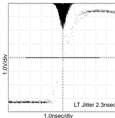
Figure 16. 24.6MHz LT Jitter V_{DD}=3.3V , at C_L=15pF
