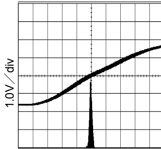
Fig.19 BUF_OUT(27MHz) Period-Jitter VDD=3.3V,CL=50pF
