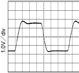
Fig.15 54MHz output waveform VDD=3.3V,CL=15pF
