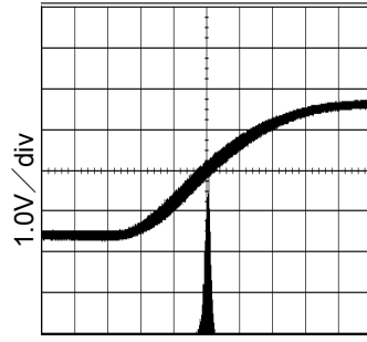
Fig.16 54MHz Period-Jitter VDD=3.3V,CL=15pF
