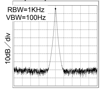
Fig.17 54MHz spectrum VDD=3.3V,CL=15pF
