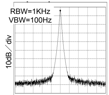
Fig.20 BUF_OUT(27MHz) spectrum VDD=3.3V,CL=50pF
