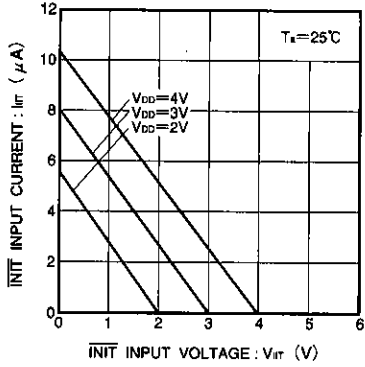
Fig. 30 \overline{\text{INIT}} input current vs. voltage characteristic (typical values)
