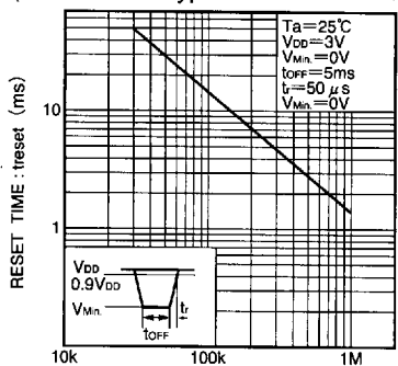
EXTERNAL CLOCK FREQUENCY : f_{ck} (Hz) (Note: There is no Power On Reset circuit in the BU2466.)
