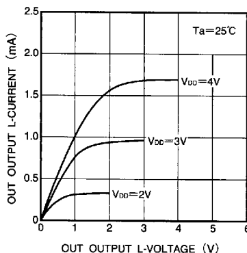
Fig. 34 OUT output "L" current characteristic (typical values)
