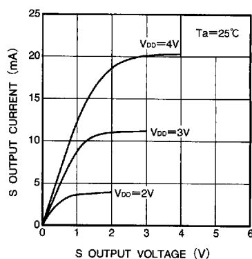
Fig. 35 S output current characteristic (typical values)
