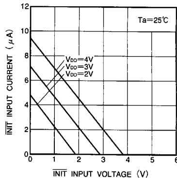
Fig. 32 \overline{INIT} input current characteristic (typical values)
