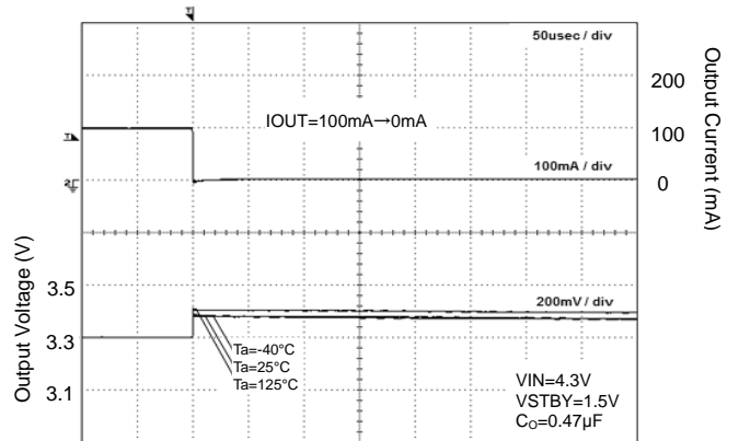
Figure 18. Load Response
