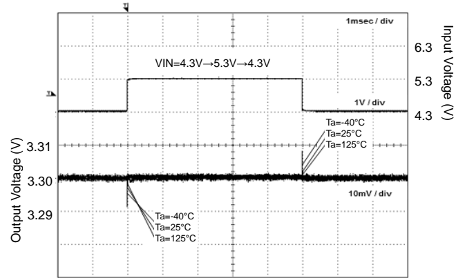
Figure 28. VIN Response
