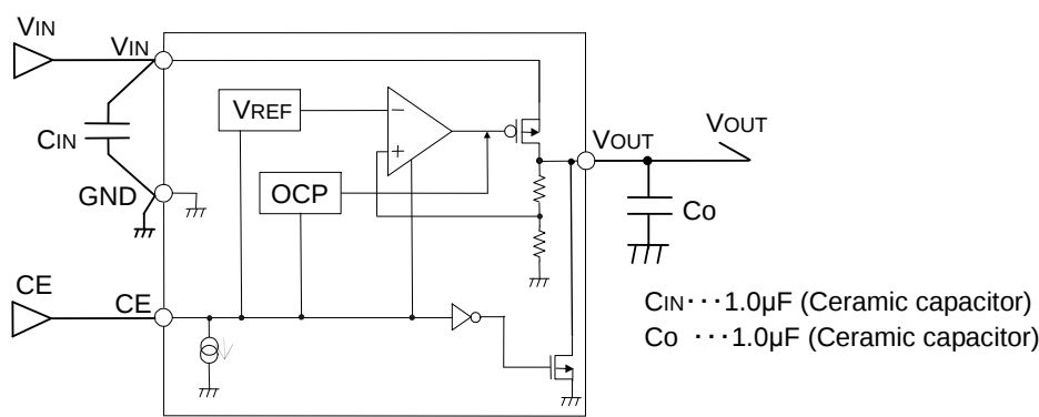
Figure 2. Block Diagrams
