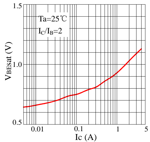
Fig6 V BESat -I C
