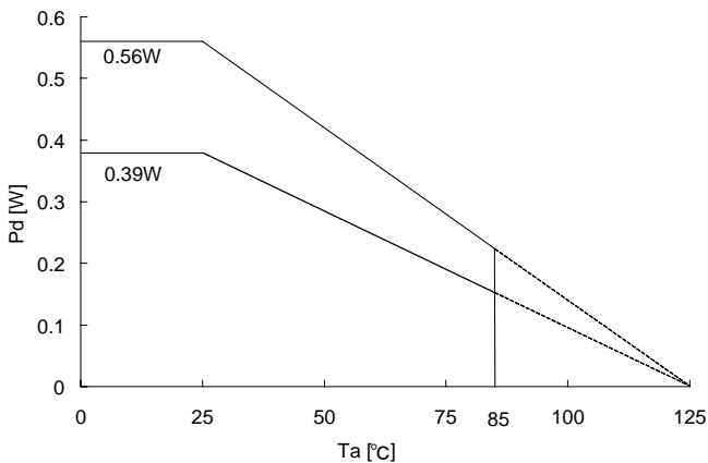
Fig. 23 SSON04X1010 Power dissipation heat reduction characteristics (Reference)
