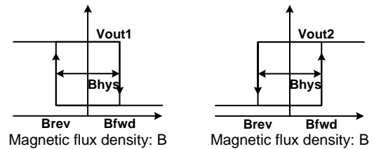
Figure 2. Output operation
