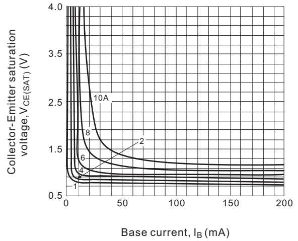
Fig.3 Collector-Emmitter saturation voltage
