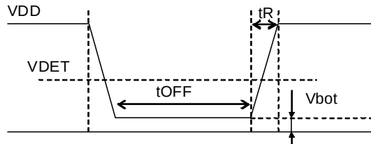
Figure 17. Power ON/OFF Waveform
