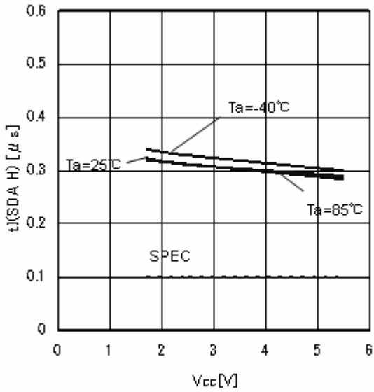
Figure 26. Noise removal time t_I (SDA H)
