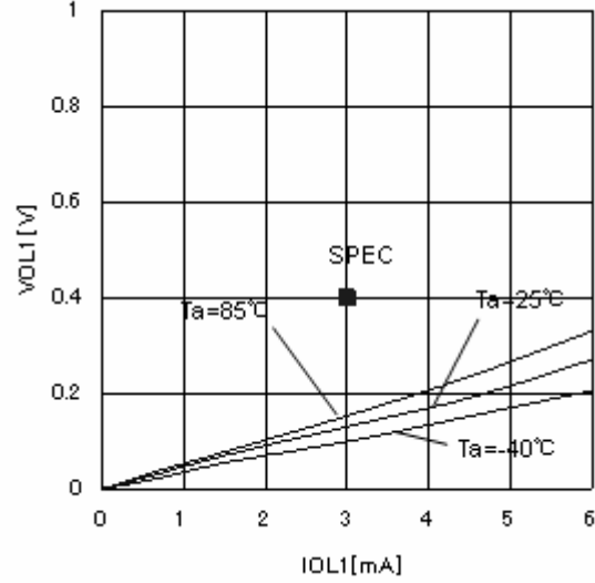
Figure 5. L input voltage V_{OL1-IOL1} ( V_{CC}=2.5V )
